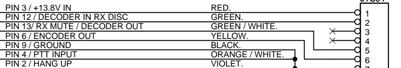
EXAMPLE 1: TS-64WDS ENCODE/DECODE ONLY WITHOUT PL FILTER OR REVERSE BURST
