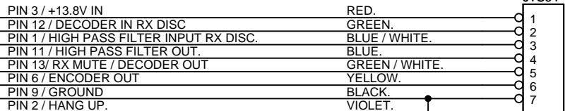
EXAMPLE 2: TS-64WDS ENCODE/DECODE WITH PL FILTER
